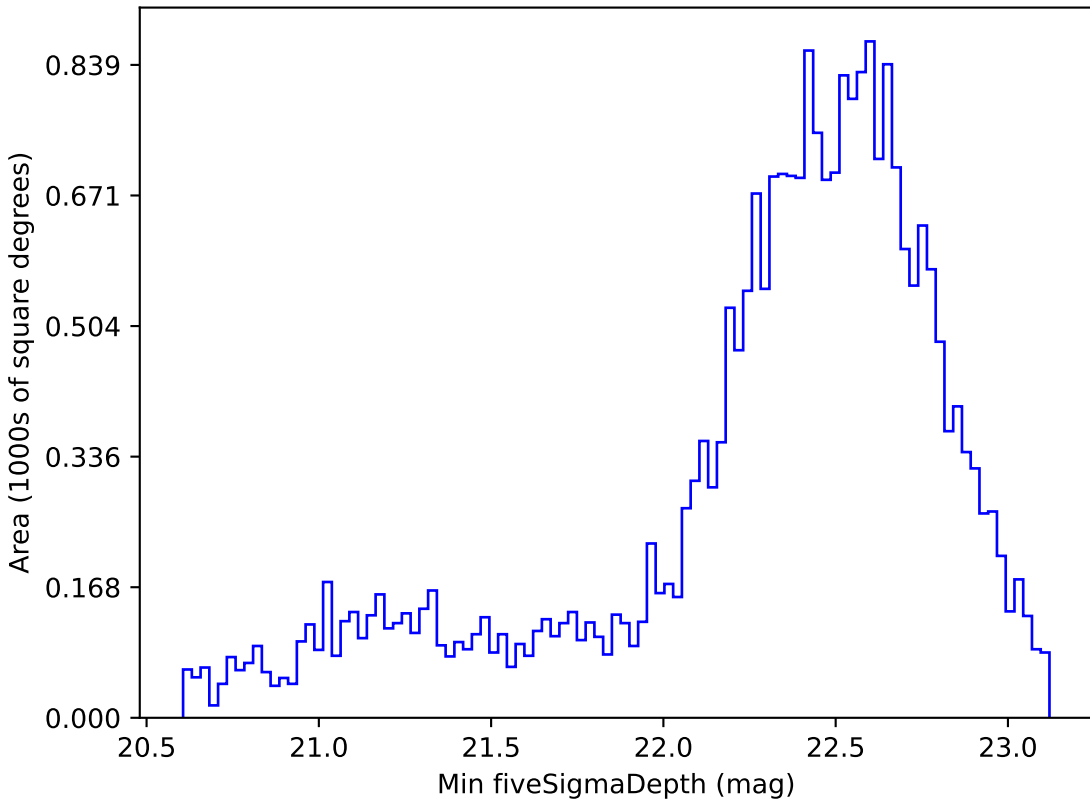
smc_lmc_v3.3_10yrs Yr 1 z band: Min fiveSigmaDepth
