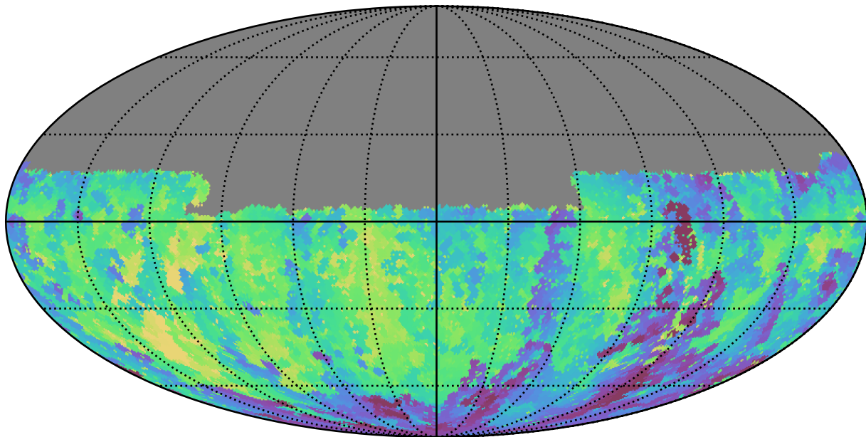
smc_lmc_v3.3_10yrs Yr 1 u band: Min fiveSigmaDepth
