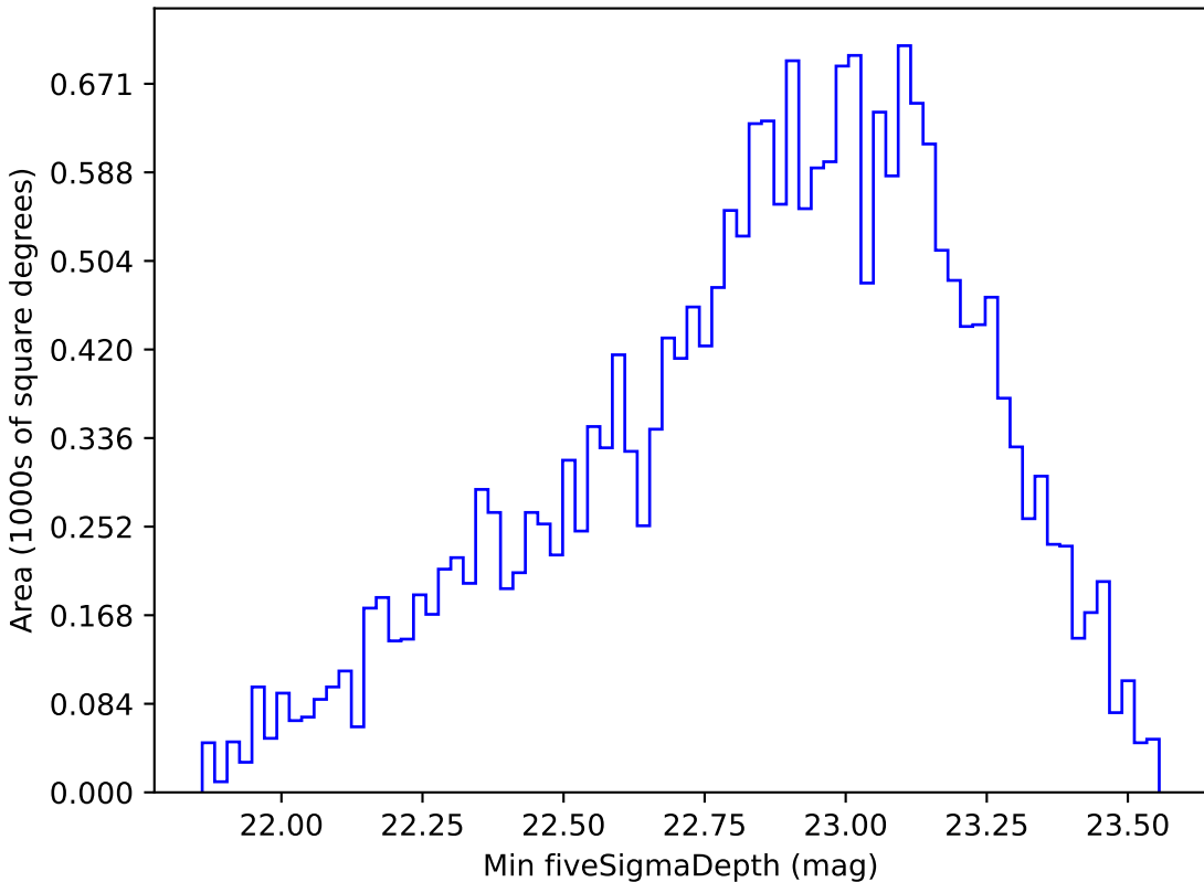
smc_lmc_v3.3_10yrs Yr 1 u band: Min fiveSigmaDepth
