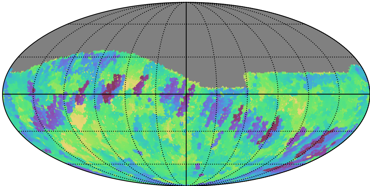
smc_lmc_v3.3_10yrs Yr 1 r band: Min fiveSigmaDepth
