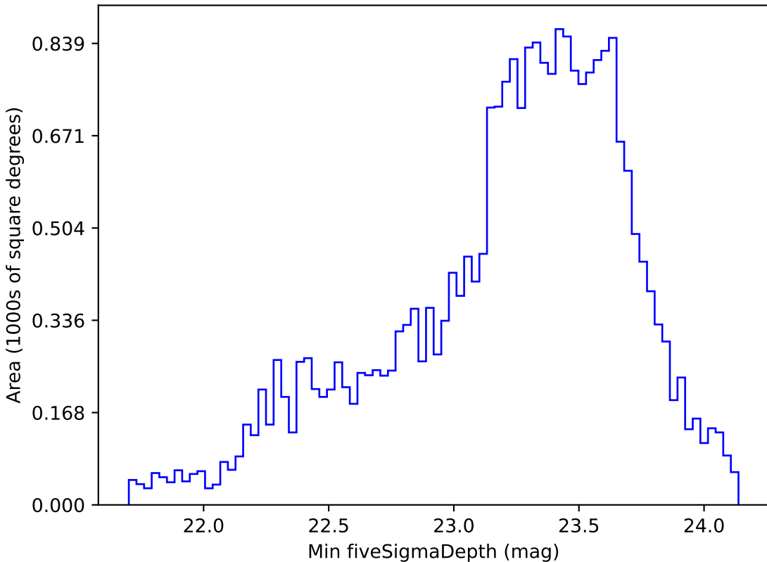
smc_lmc_v3.3_10yrs Yr 1 r band: Min fiveSigmaDepth
