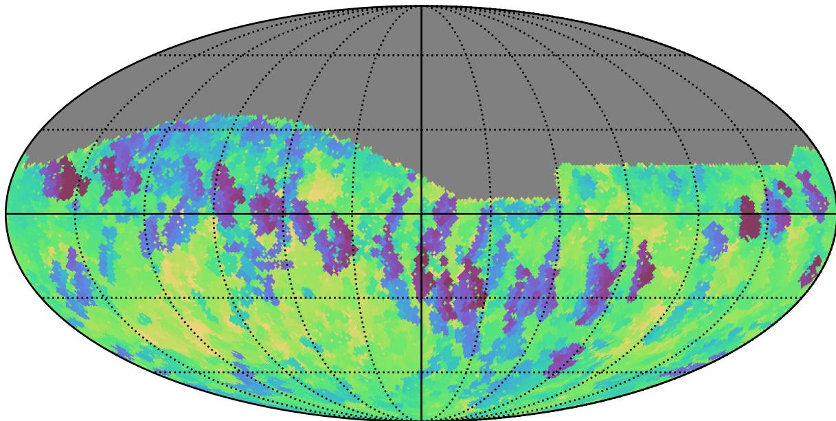
smc_lmc_v3.3_10yrs Yr 1 i band: Min fiveSigmaDepth
