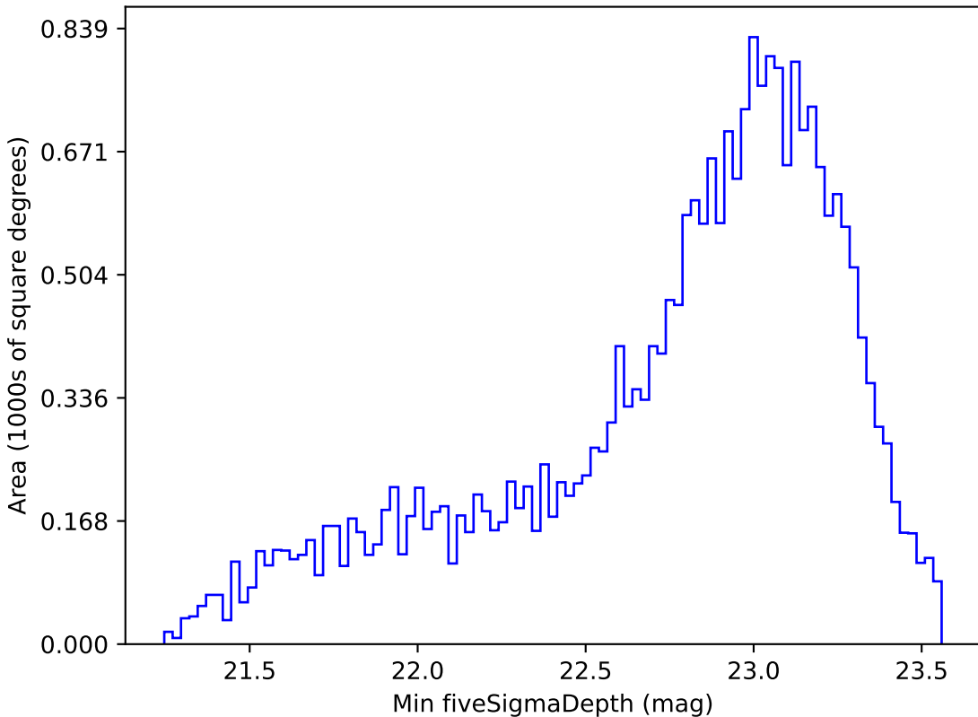
smc_lmc_v3.3_10yrs Yr 1 i band: Min fiveSigmaDepth
