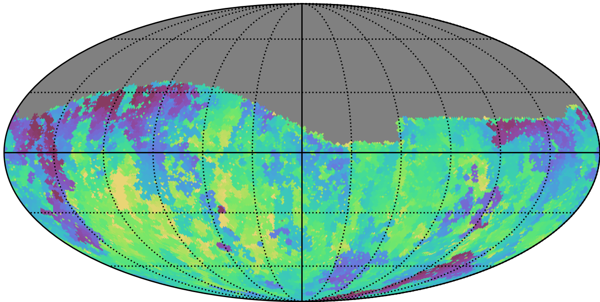
smc_lmc_v3.3_10yrs Yr 1 g band: Min fiveSigmaDepth
