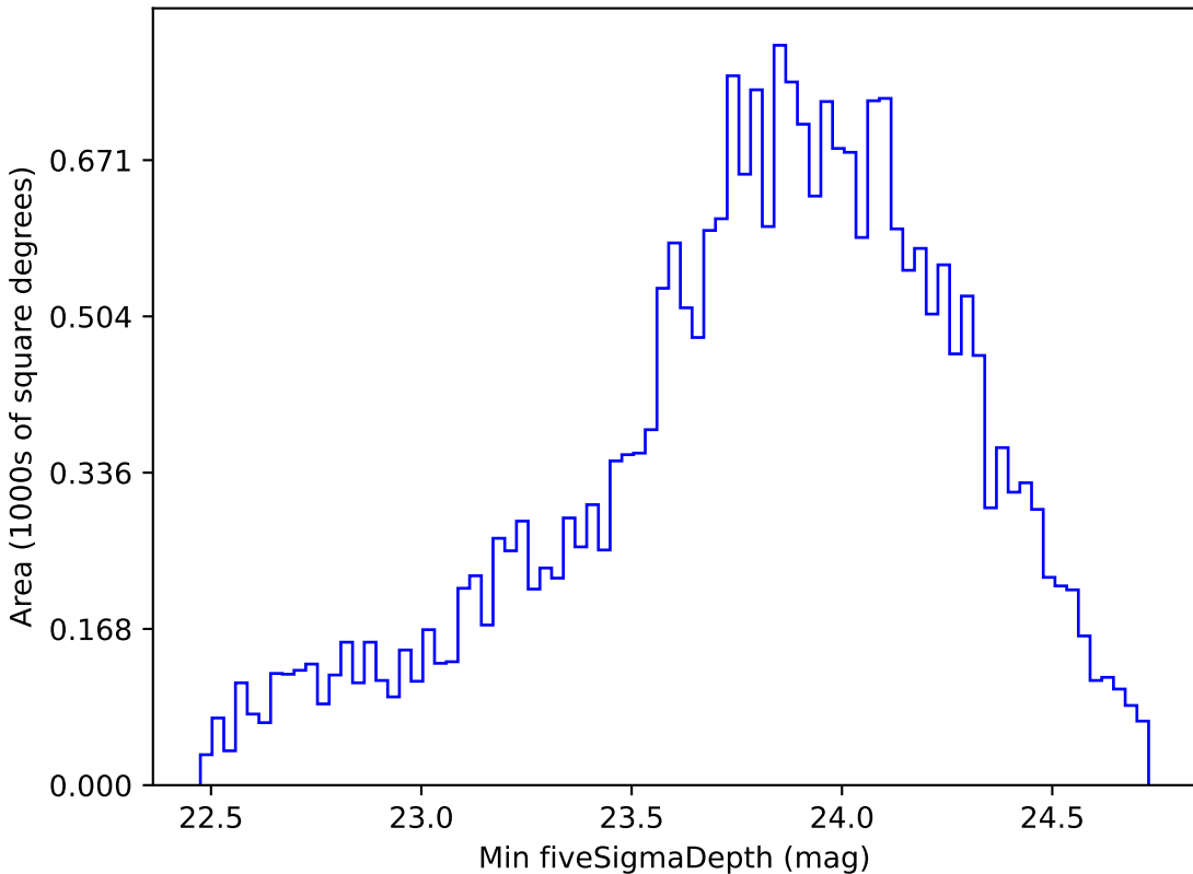
smc_lmc_v3.3_10yrs Yr 1 g band: Min fiveSigmaDepth
