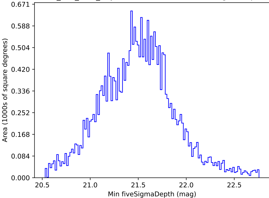
smc_lmc_v3.3_10yrs Yr 1 all bands: Min fiveSigmaDepth
