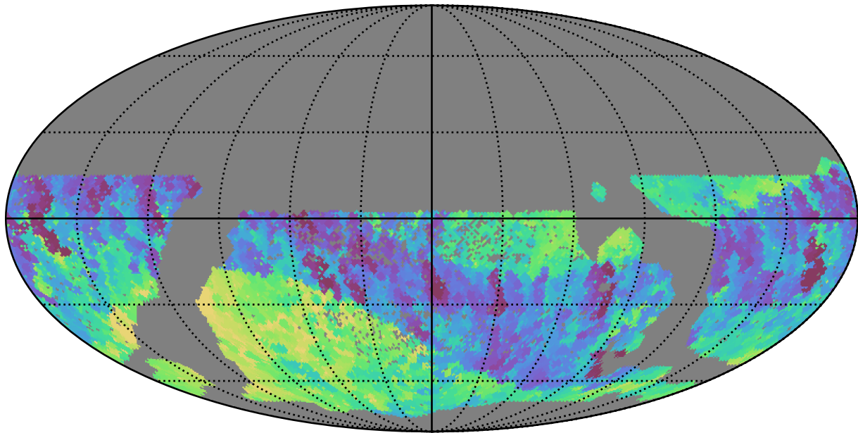
smc_lmc_v3.3_10yrs WFD z band: Min fiveSigmaDepth
