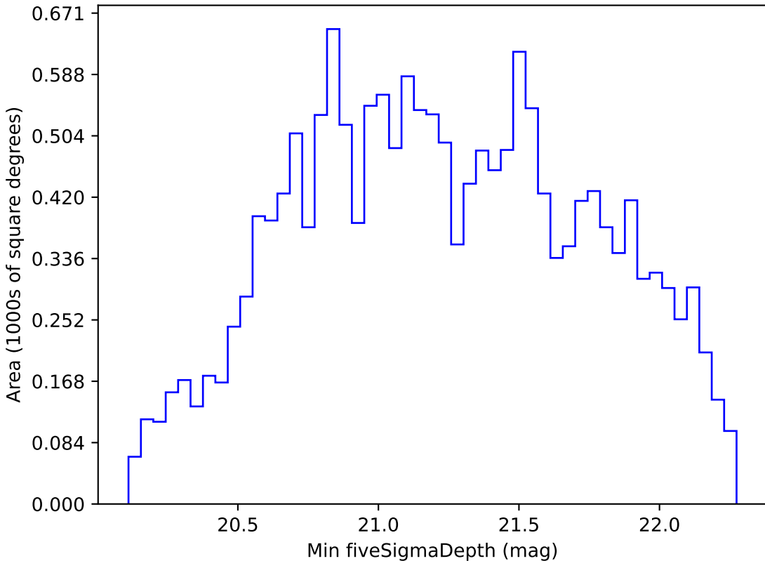
smc_lmc_v3.3_10yrs WFD z band: Min fiveSigmaDepth
