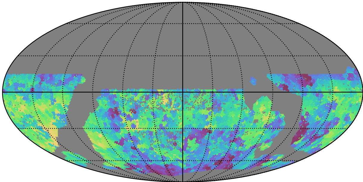
smc_lmc_v3.3_10yrs WFD u band: Min fiveSigmaDepth
