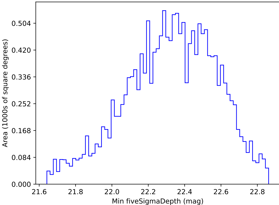
smc_lmc_v3.3_10yrs WFD u band: Min fiveSigmaDepth
