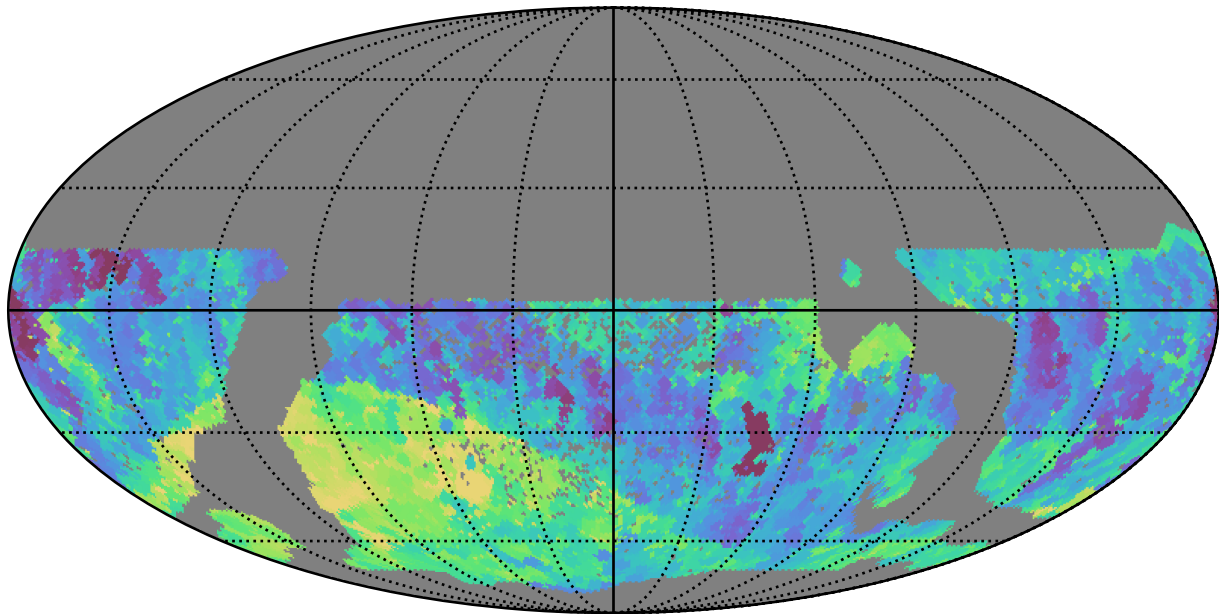
smc_lmc_v3.3_10yrs WFD i band: Min fiveSigmaDepth
