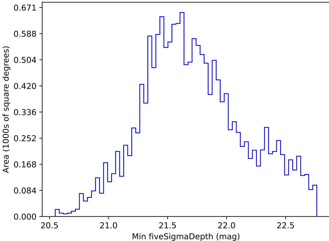
smc_lmc_v3.3_10yrs WFD i band: Min fiveSigmaDepth
