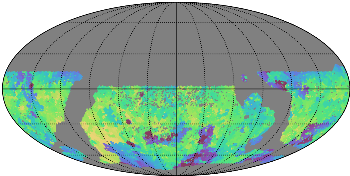
smc_lmc_v3.3_10yrs WFD g band: Min fiveSigmaDepth
