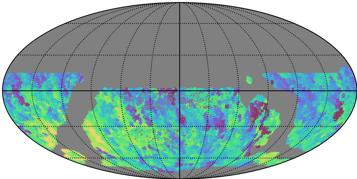
smc_lmc_v3.3_10yrs WFD all bands: Min fiveSigmaDepth
