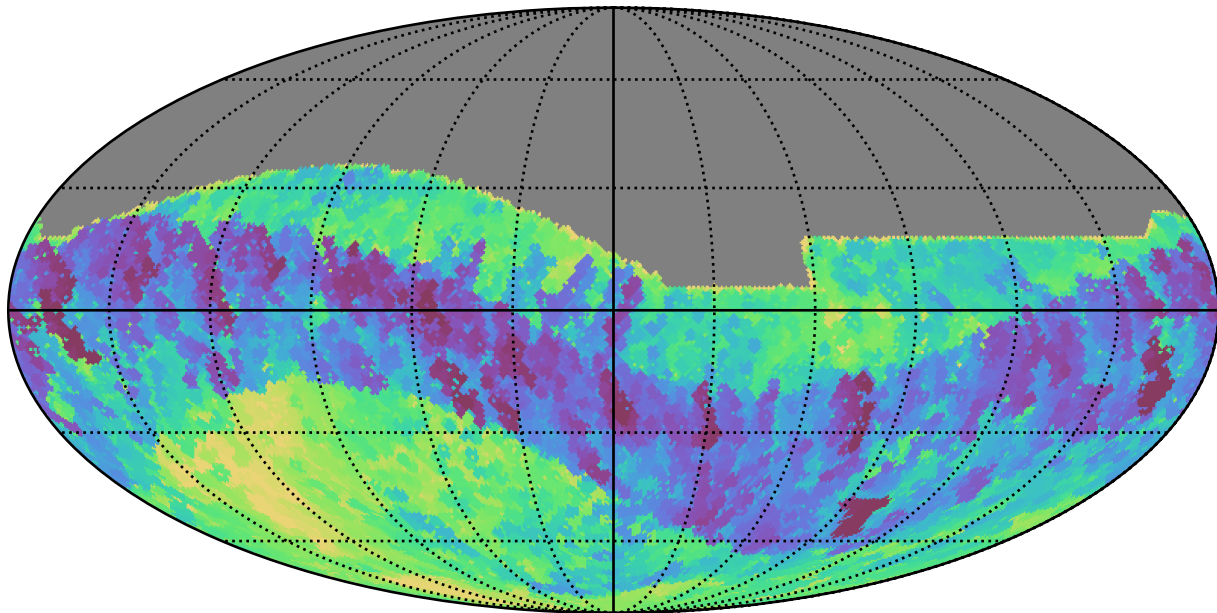
smc_lmc_v3.3_10yrs All sky z band: Min fiveSigmaDepth
