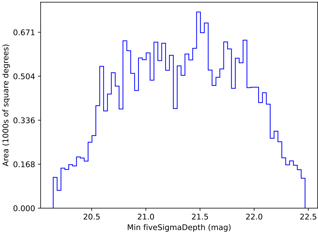
smc_lmc_v3.3_10yrs All sky z band: Min fiveSigmaDepth
