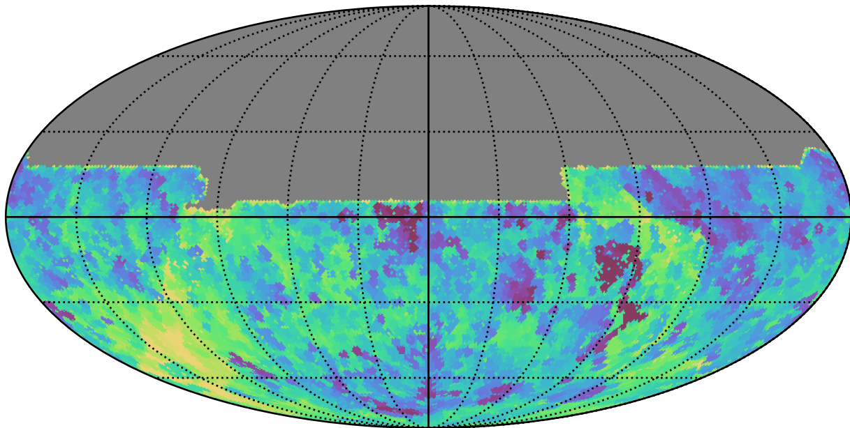
smc_lmc_v3.3_10yrs All sky y band: Min fiveSigmaDepth
