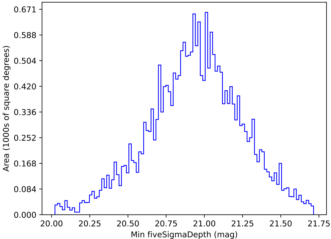
smc_lmc_v3.3_10yrs All sky y band: Min fiveSigmaDepth
