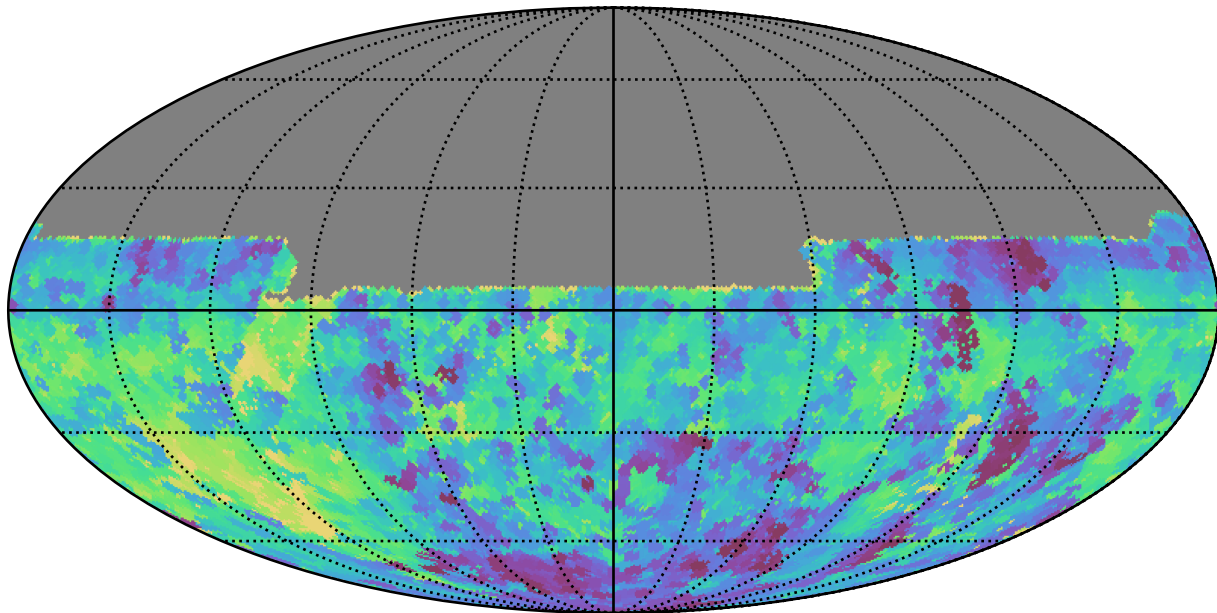
smc_lmc_v3.3_10yrs All sky u band: Min fiveSigmaDepth
