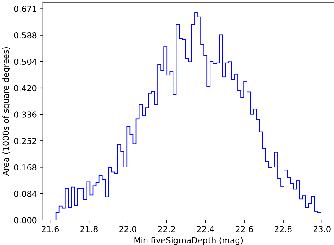
smc_lmc_v3.3_10yrs All sky u band: Min fiveSigmaDepth
