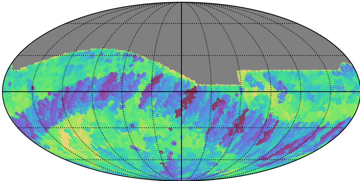
smc_lmc_v3.3_10yrs All sky r band: Min fiveSigmaDepth
