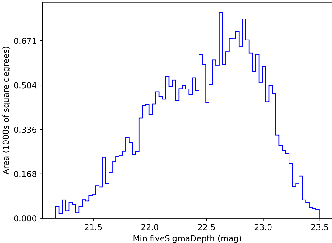
smc_lmc_v3.3_10yrs All sky r band: Min fiveSigmaDepth
