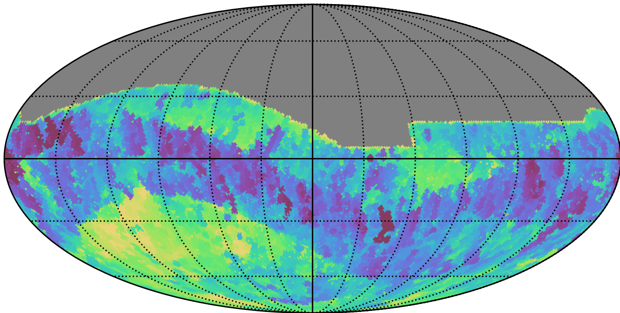
smc_lmc_v3.3_10yrs All sky i band: Min fiveSigmaDepth
