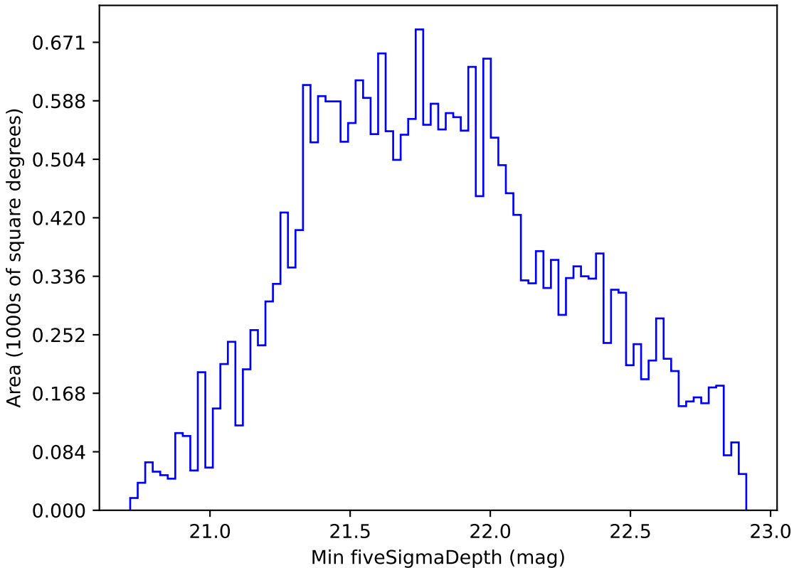
smc_lmc_v3.3_10yrs All sky i band: Min fiveSigmaDepth
