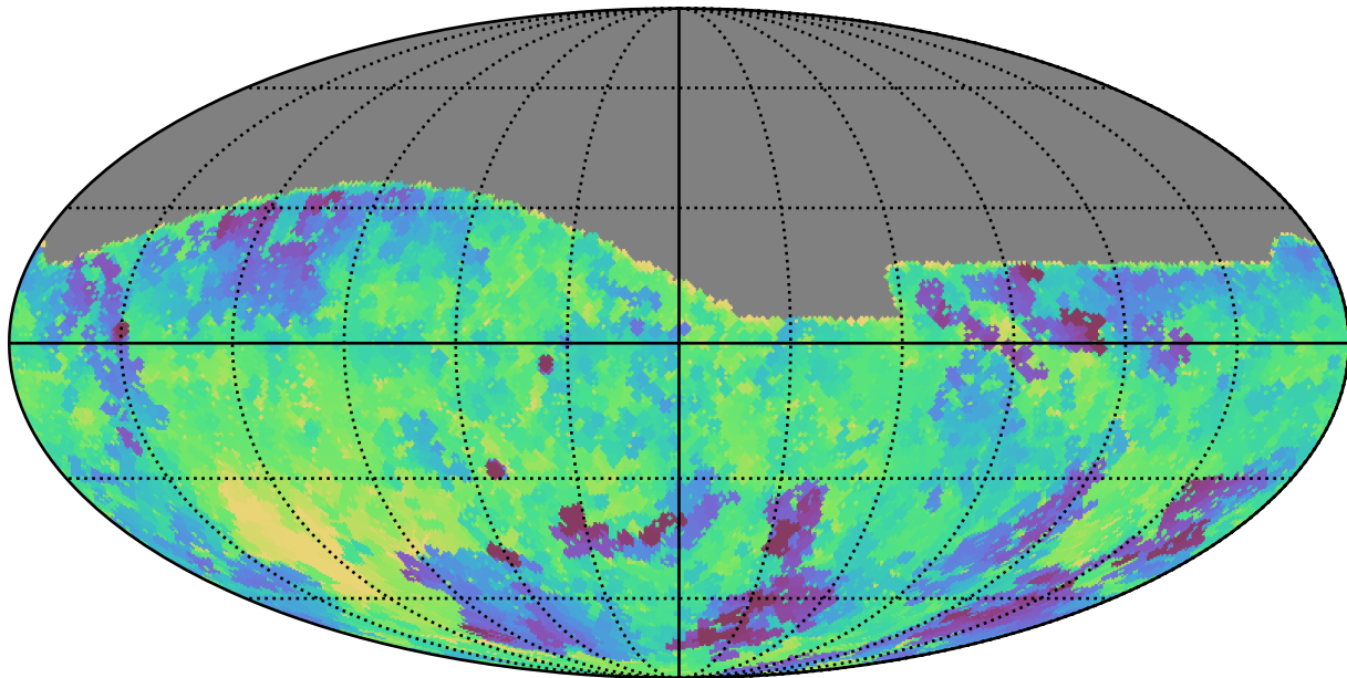
smc_lmc_v3.3_10yrs All sky g band: Min fiveSigmaDepth
