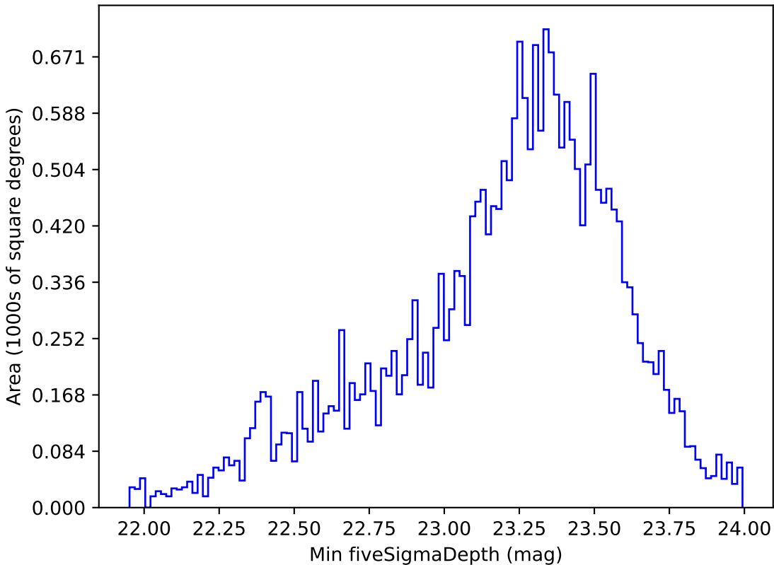
smc_lmc_v3.3_10yrs All sky g band: Min fiveSigmaDepth
