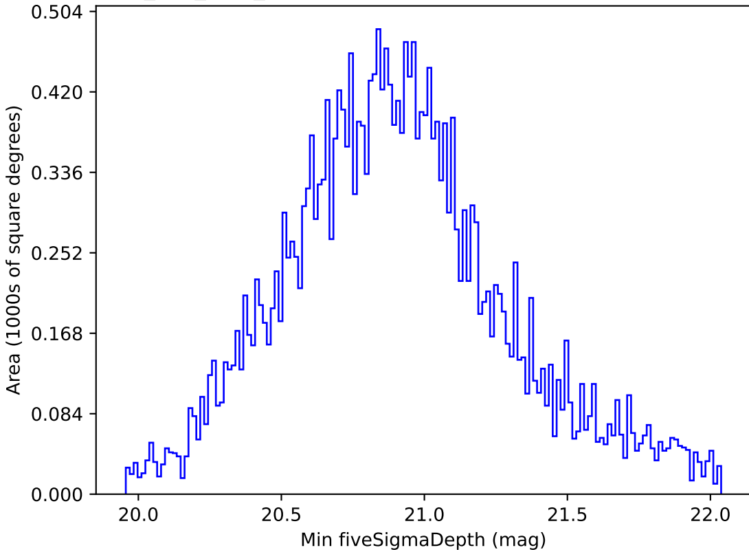
smc_lmc_v3.3_10yrs All sky all bands: Min fiveSigmaDepth
