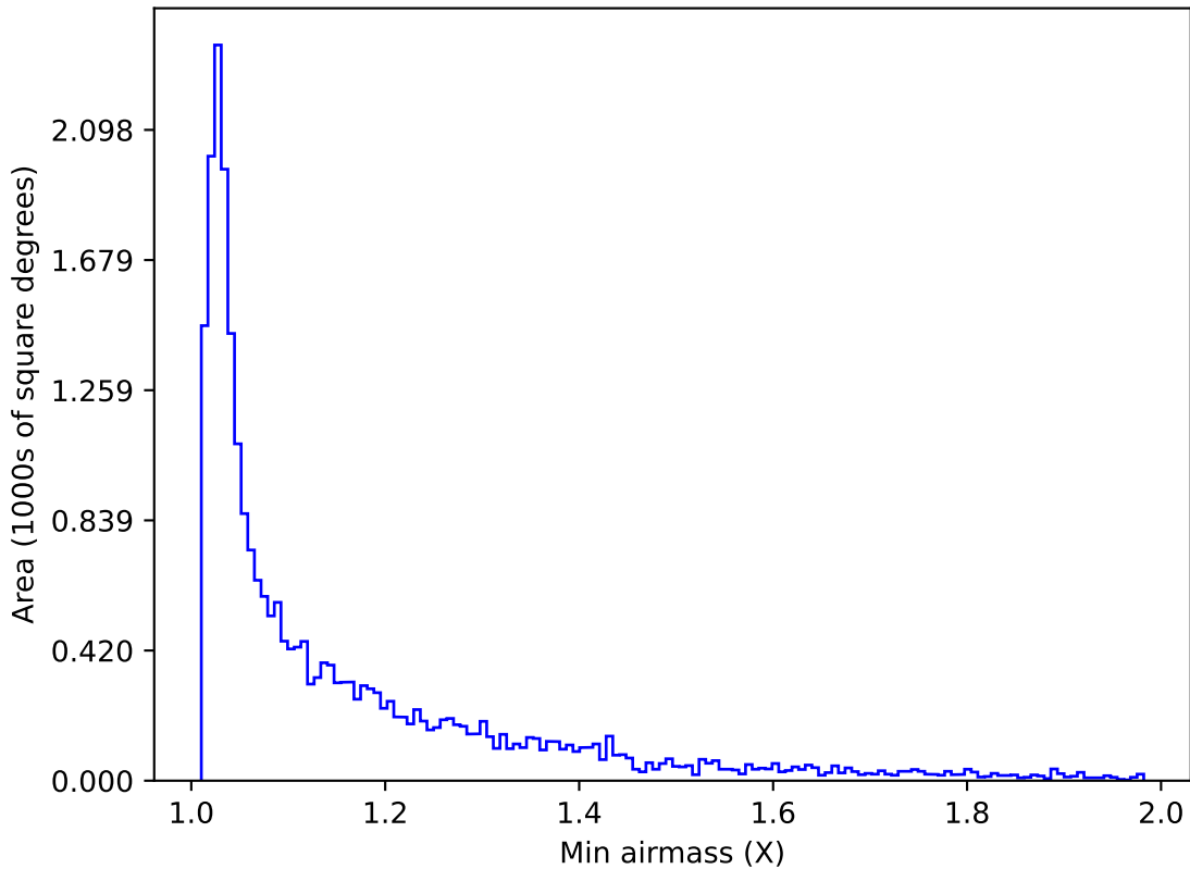
smc_lmc_v3.3_10yrs Yr 1 z band: Min airmass
