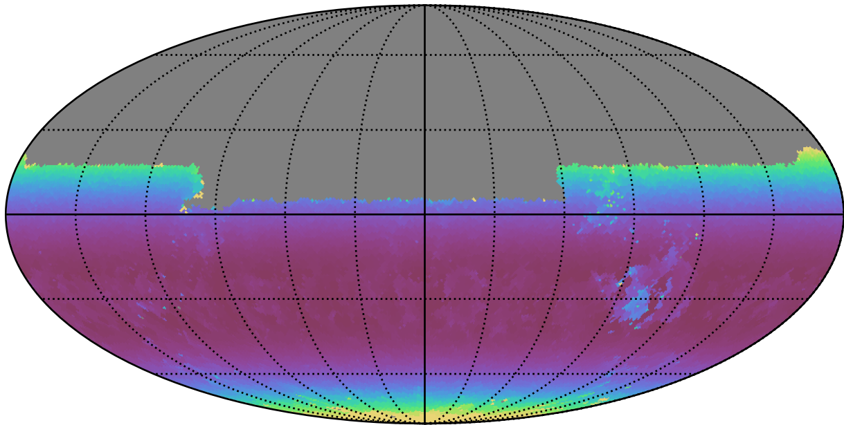
smc_lmc_v3.3_10yrs Yr 1 y band: Min airmass
