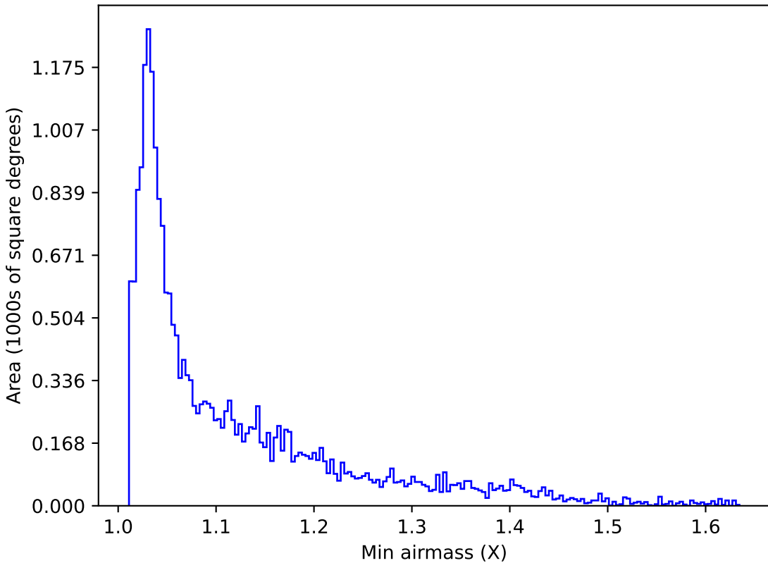
smc_lmc_v3.3_10yrs Yr 1 y band: Min airmass
