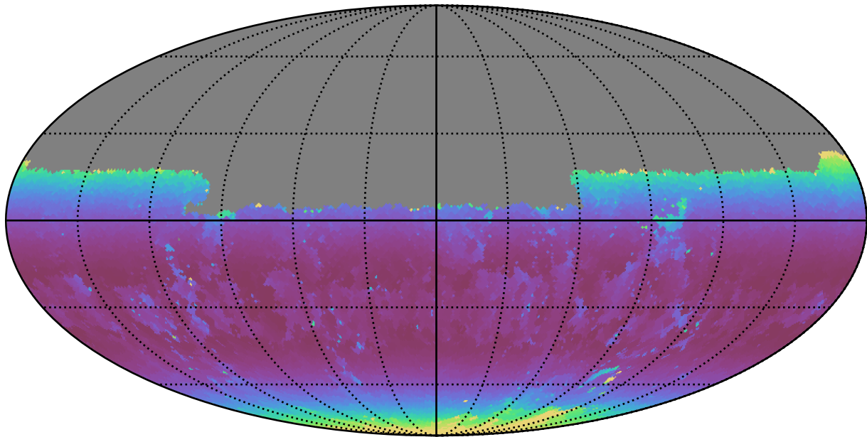
smc_lmc_v3.3_10yrs Yr 1 u band: Min airmass
