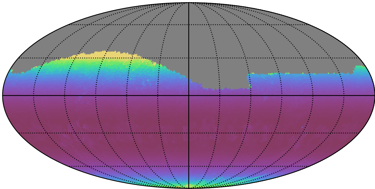
smc_lmc_v3.3_10yrs Yr 1 r band: Min airmass
