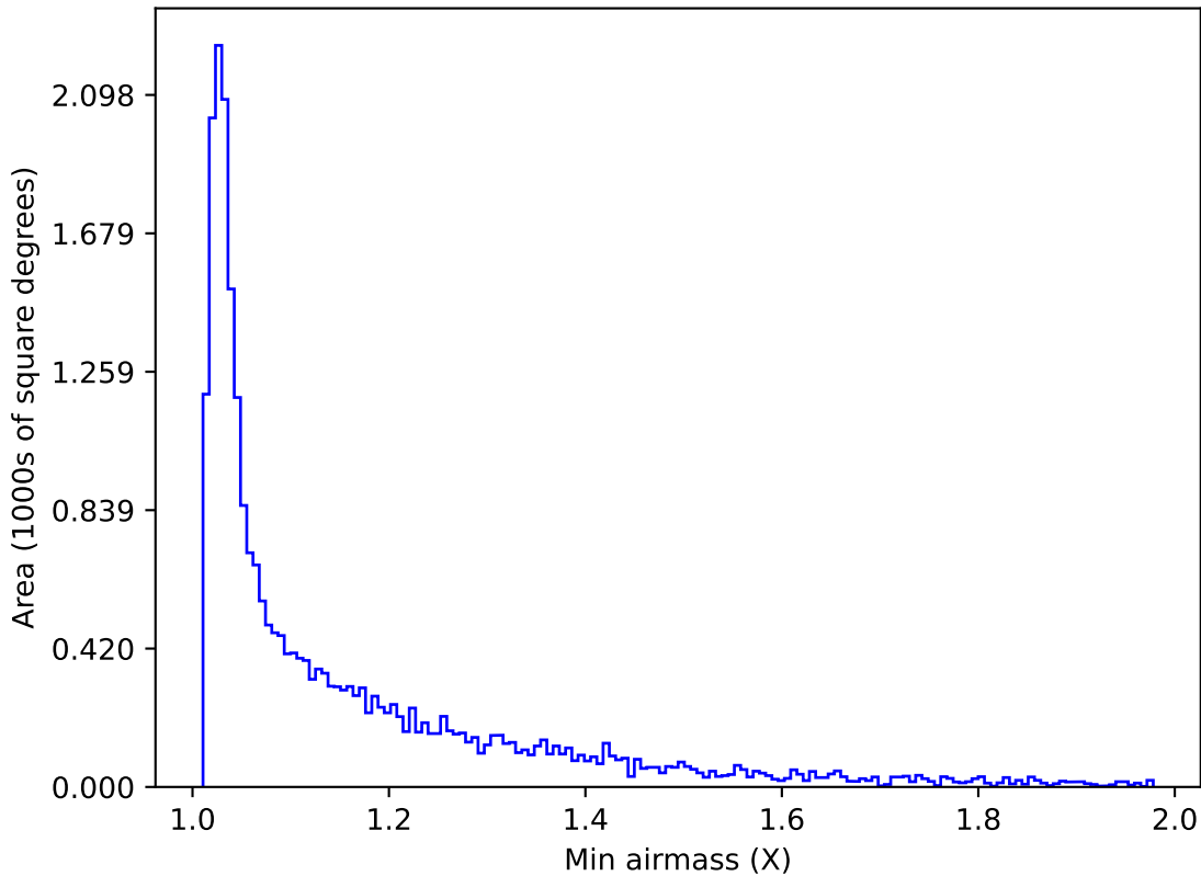
smc_lmc_v3.3_10yrs Yr 1 r band: Min airmass
