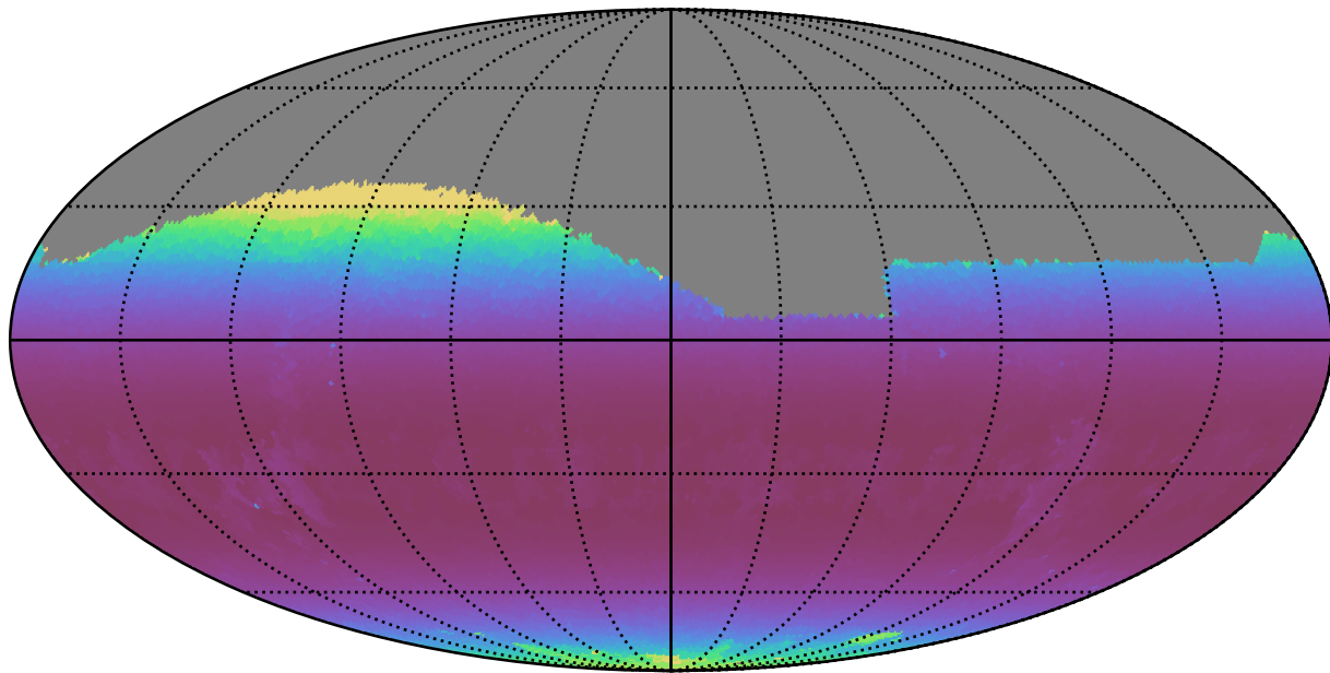
smc_lmc_v3.3_10yrs Yr 1 i band: Min airmass
