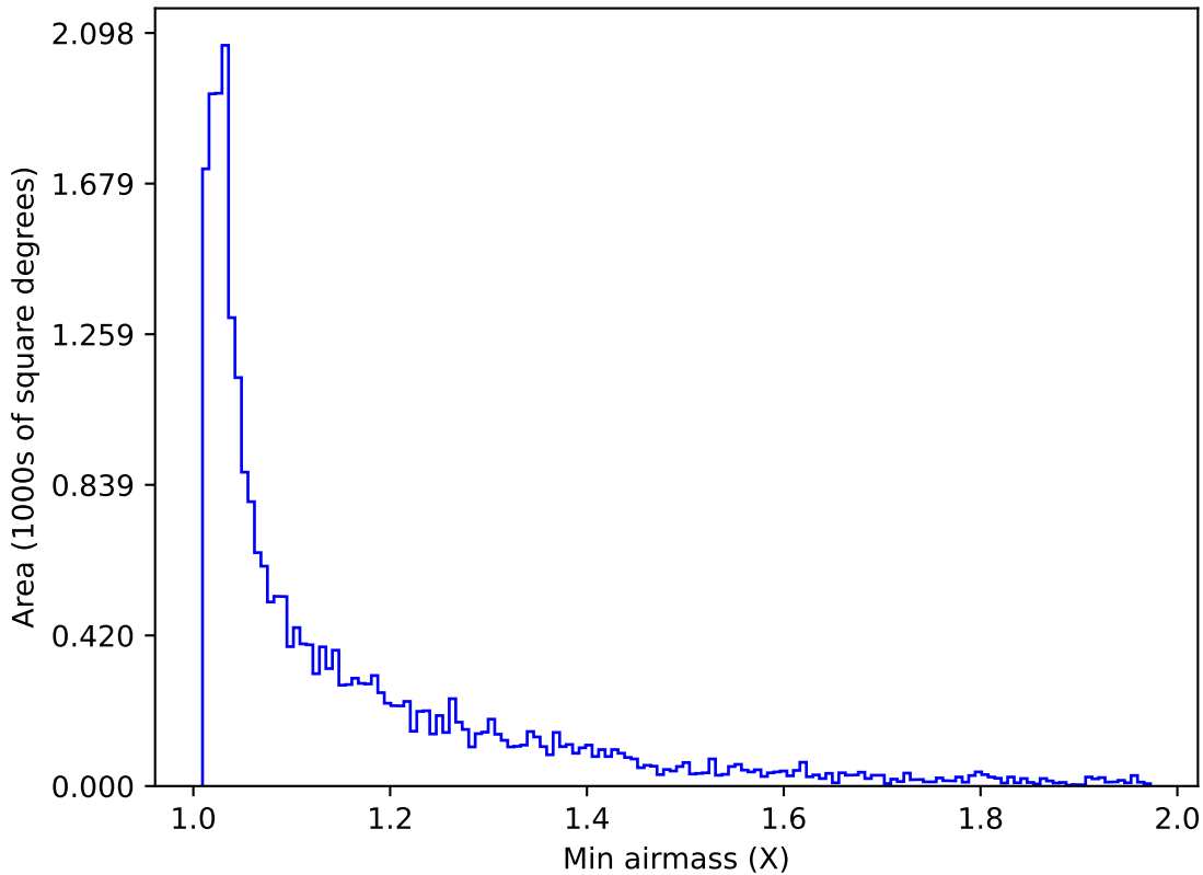
smc_lmc_v3.3_10yrs Yr 1 i band: Min airmass
