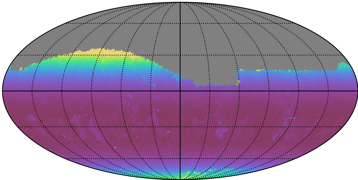
smc_lmc_v3.3_10yrs Yr 1 g band: Min airmass
