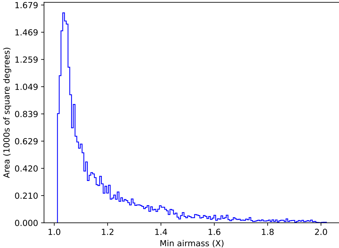
smc_lmc_v3.3_10yrs Yr 1 g band: Min airmass
