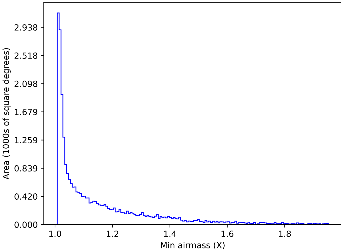
smc_lmc_v3.3_10yrs Yr 1 all bands: Min airmass
