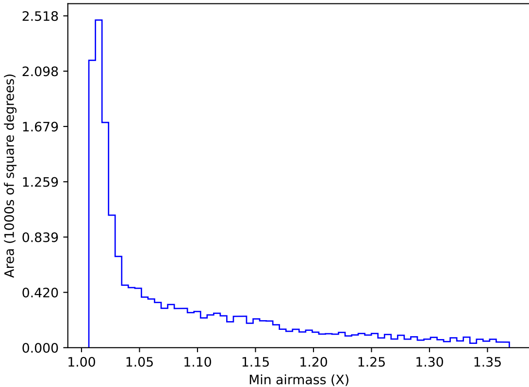
smc_lmc_v3.3_10yrs WFD z band: Min airmass
