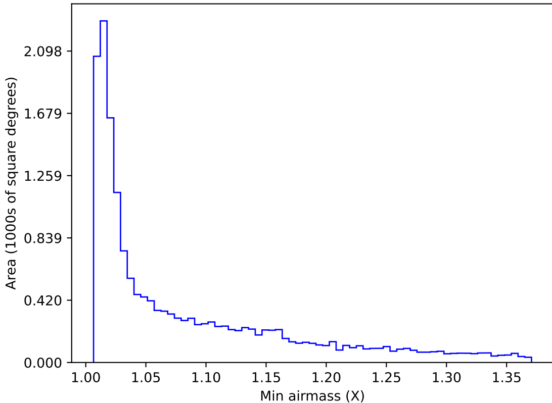
smc_lmc_v3.3_10yrs WFD y band: Min airmass
