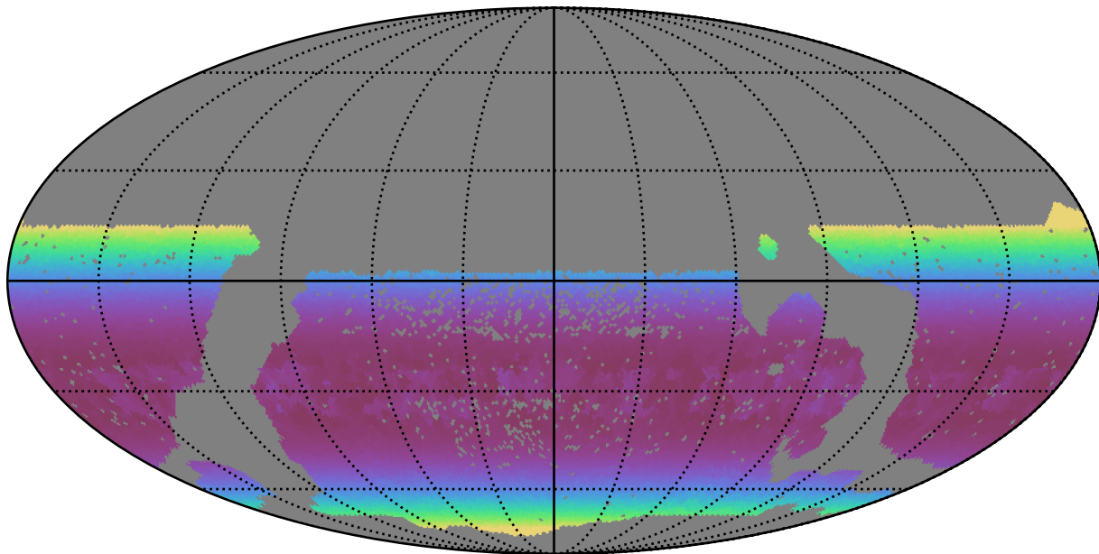
smc_lmc_v3.3_10yrs WFD u band: Min airmass
