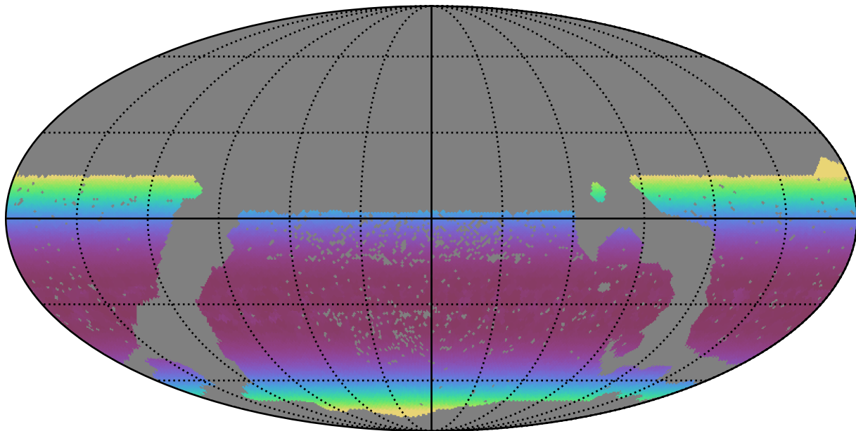
smc_lmc_v3.3_10yrs WFD r band: Min airmass
