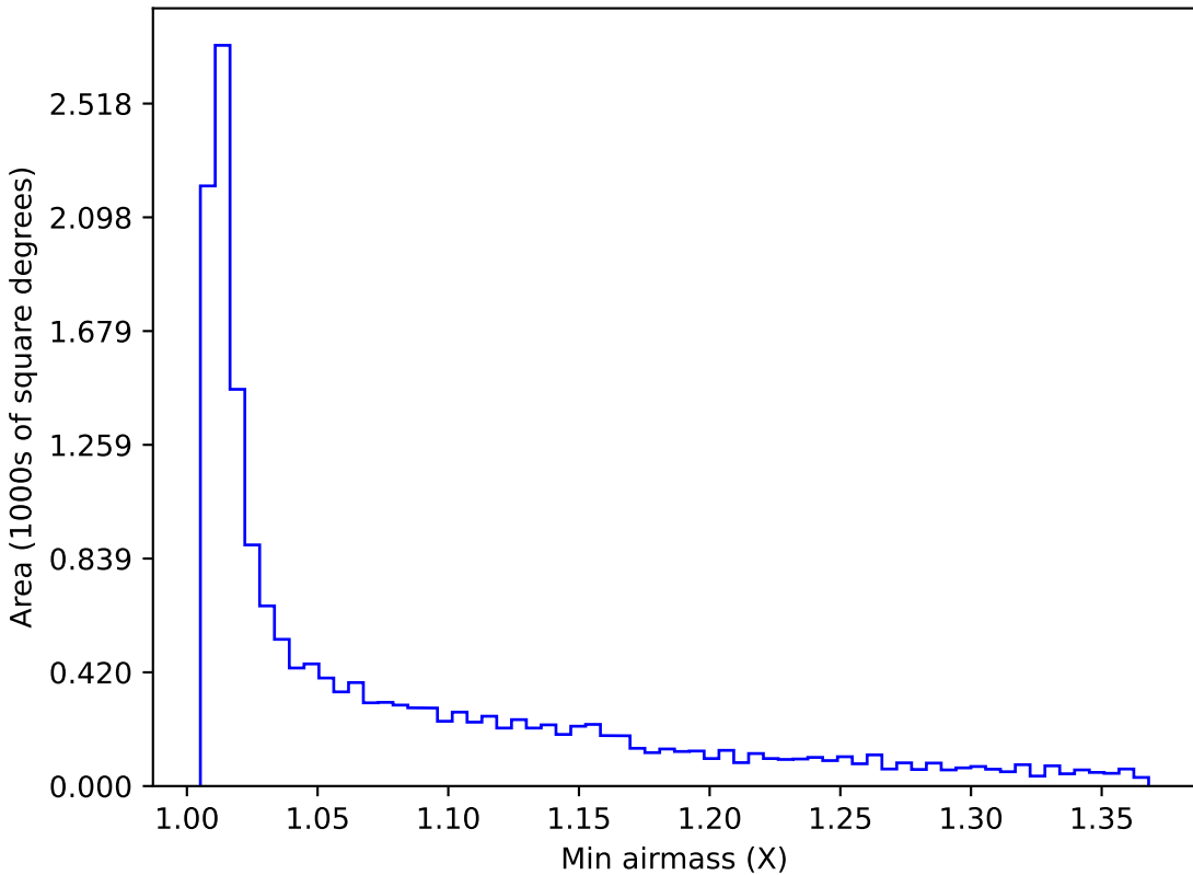
smc_lmc_v3.3_10yrs WFD r band: Min airmass
