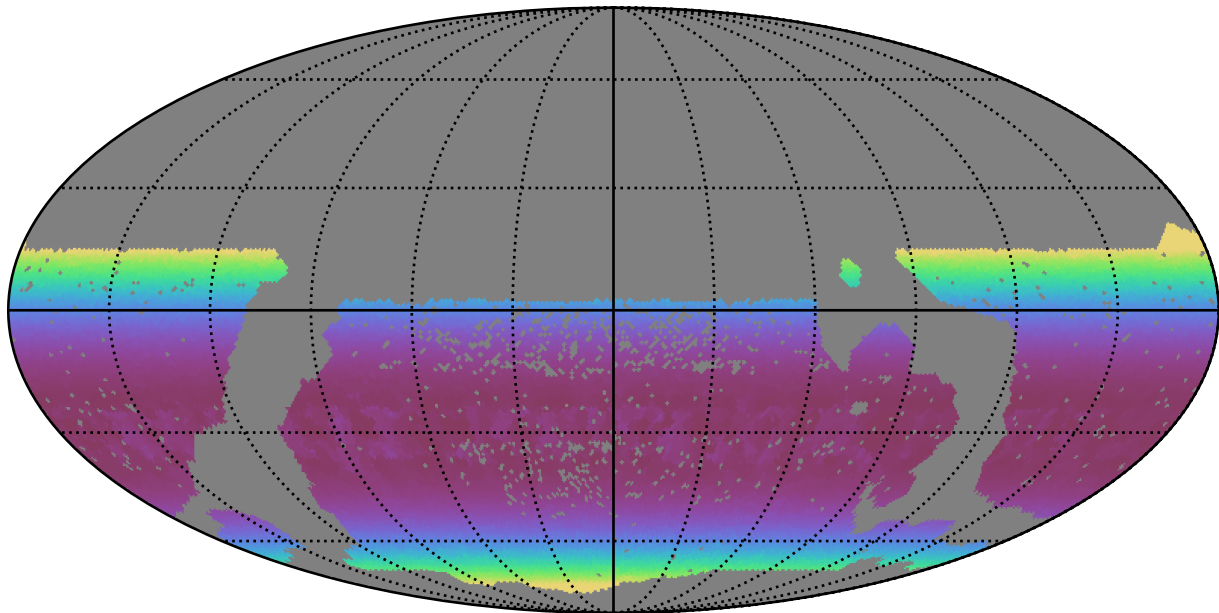
smc_lmc_v3.3_10yrs WFD g band: Min airmass
