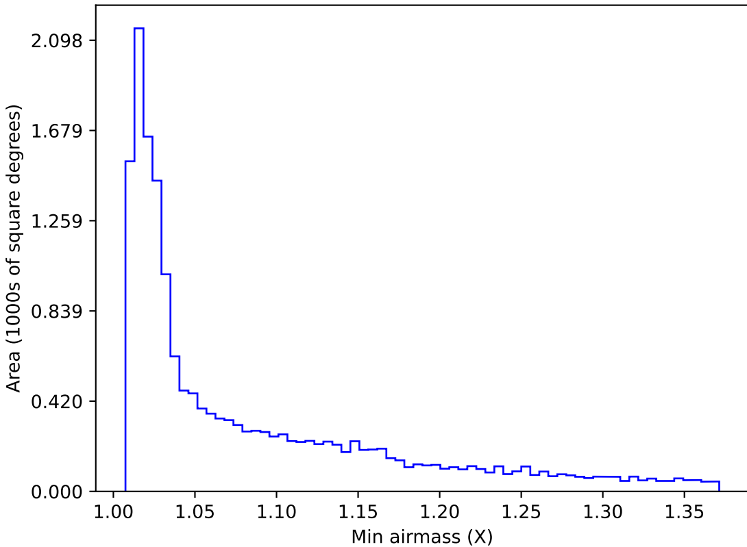
smc_lmc_v3.3_10yrs WFD g band: Min airmass
