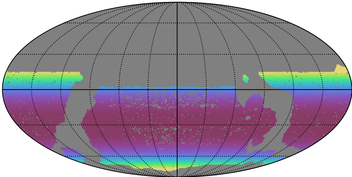
smc_lmc_v3.3_10yrs WFD all bands: Min airmass
